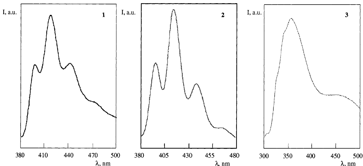
Figure 2. Emission spectra in acetonitrile solution of 1 (left), 2 (middle), and 3 (right); excitation wavelength is 260 nm in all the cases
