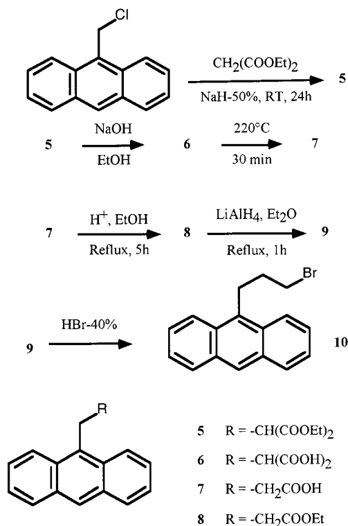
Scheme 2. Synthesis of 9-(3-bromopropyl)anthracene
