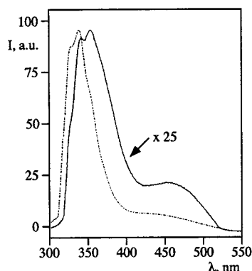
Figure 5. Normalized emission spectra of unprotonated (solid line) and protonated (dashed line) 3
