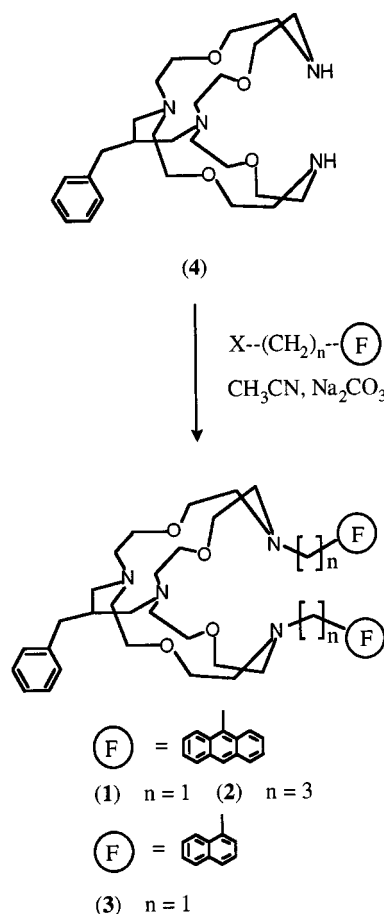
Scheme 1. Synthesis of receptors 1–3
