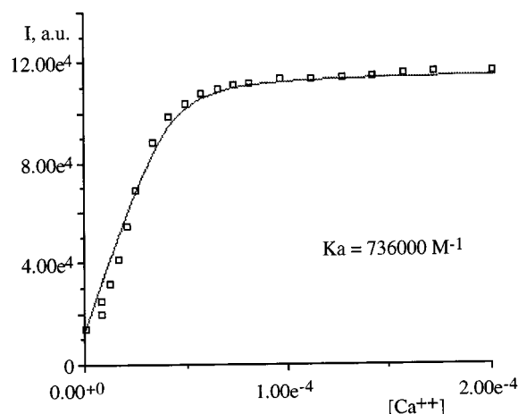
Figure 6. Luminescence output changes and best fitting of the data for 3 and \text{Ca}^{2+} ; the fitting was obtained from Equation (1) (see text)
