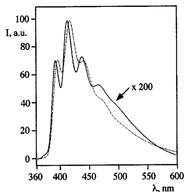
Figure 4. Normalized emission spectra of unprotonated (solid line) and protonated (dashed line) 1
