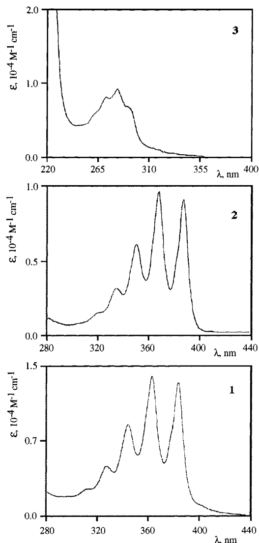
Figure 1. Absorption spectra in acetonitrile solution of 1 , 2 , and 3
